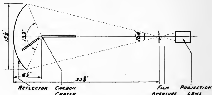
FIG. 3. Diagram of the f/2.0 reflector arc system.
